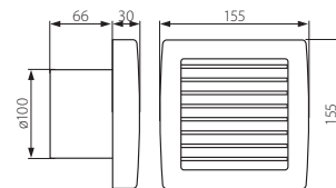
TWISTER AOL100
