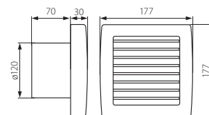
TWISTER AOL120
